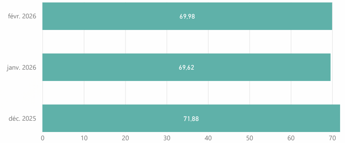
Dwell time
